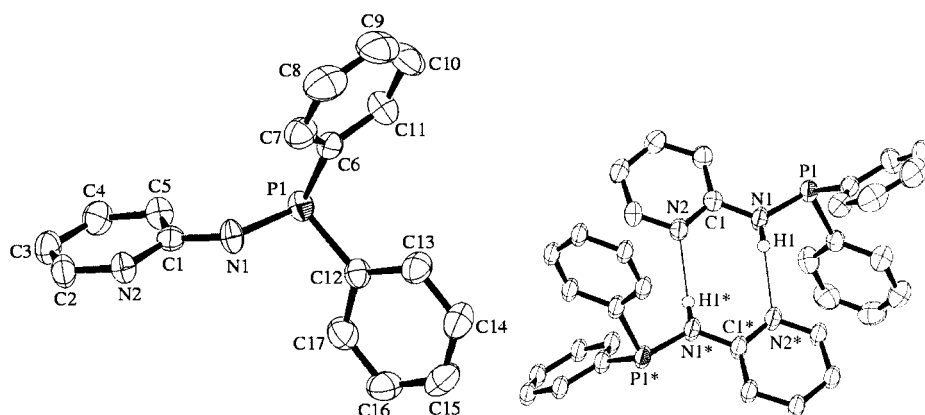
Figure 2. Crystal structure of complex 1 and its dimer in the crystal structure ( N1-N2^* = 3.050 \text{ \AA} and H1-N2^* = 2.18 \text{ \AA} ); thermal ellipsoids given at 50% probability
