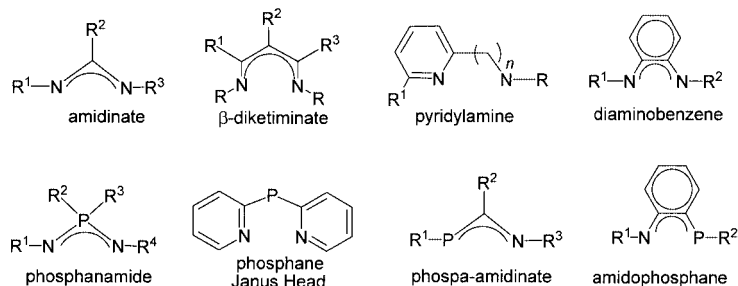
Scheme 1. Representative P,N - and N,N -ancillary ligations in lithium complexes
