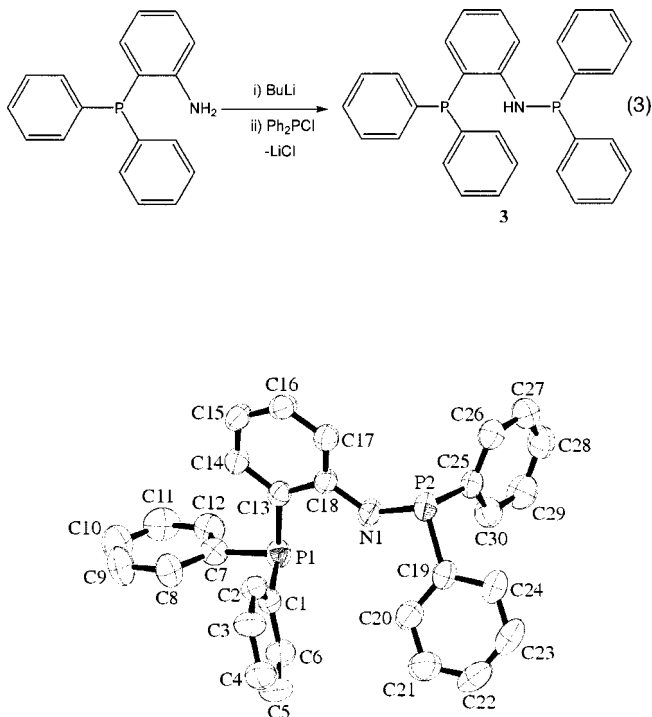
Figure 4. Molecular structure of compound 3 ; thermal ellipsoids given at 50% probability
