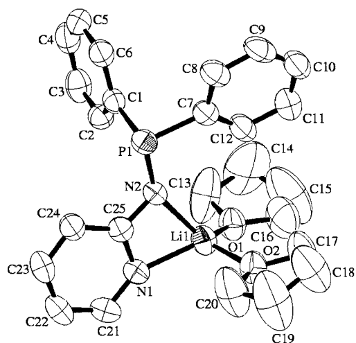
Figure 3. Molecular structure of complex 2 ; thermal ellipsoids given at 50% probability
