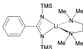
Figure 1. Lithium benzamidinate complex with TMEDA ligation
