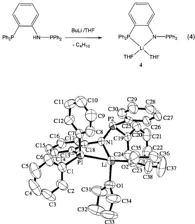
Figure 5. Molecular structure of complex 4 ; thermal ellipsoids given at 50% probability
